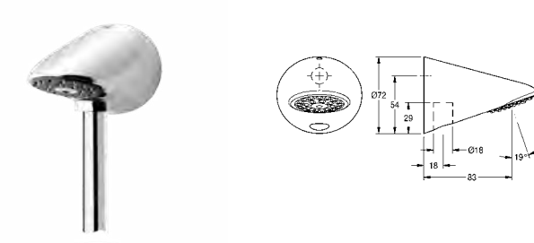
AQUAJET-SLIMLINE SHOWERHEAD BOTTOM INLET AQUAJET-Slimline showerhead DN 15 with plastic jet face with anti-calcification system and low aerosol formation, for surface pipe mounting, polished chromium-plated brass. With flow controllers 9.0 l/min and 12.0 l/min. Spout projection: 83mm Head Dimensions: 72 x 72 x 83mm AQUA757 Aquajet - slimline showerhead Mandatory accessories: ACSX2001 Shower pipe F3SV2001 Self-closing shower
