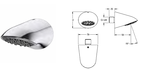
AQUAJET-SLIMLINE SHOWERHEAD FOR WALL CONNECTION AQUAJET-Slimline showerhead DN 15 with plastic jet face with anti-calcification system and low aerosol formation, for wall connection, polished chromium-plated brass. With flow controller 9.0 l/min. AQUA751 Aquajet - slimline showerhead Mandatory accessories: ESHHE0002 Flow controller 12.0l/Min
