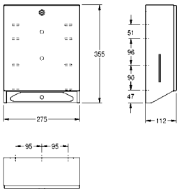
RODX600 Rodan paper towel dispenser
