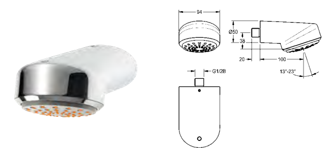
AQUAJET-COMFORT SHOWERHEAD FOR WALL CONNECTION AQUAJET-Comfort DN 15 showerhead with plastic jet face continuously adjustable between 13–23°, anti-limescale system and low aerosol formation. For wall connector with insertable connecting nozzle, diameter 26mm, high-polished chrome-plated brass housing, with integrated flow regulator 9.0l/min, ready for installation of anti-twist protection. Also suitable for shower trays, 800 x 800mm SHAC0013 Aquajet - comfort showerhead
