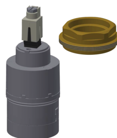
Ceramic disc cartridge with thermostatic scald-protection
