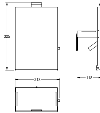
FRONT WITH WHITE SAFETY GLASS
