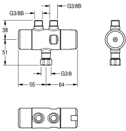
THERMOSTATIC MIXING VALVE
