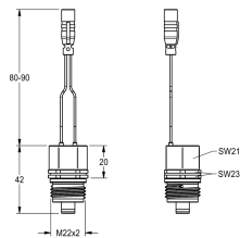
SOLENOID VALVE CARTRIDGE
