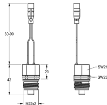
SOLENOID VALVE CARTRIDGE
