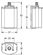
BATTERY COMPARTMENT
