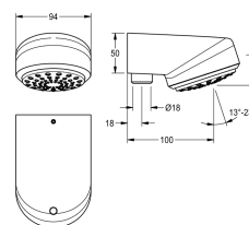
SHOWER HEAD
