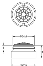
AERATOR
